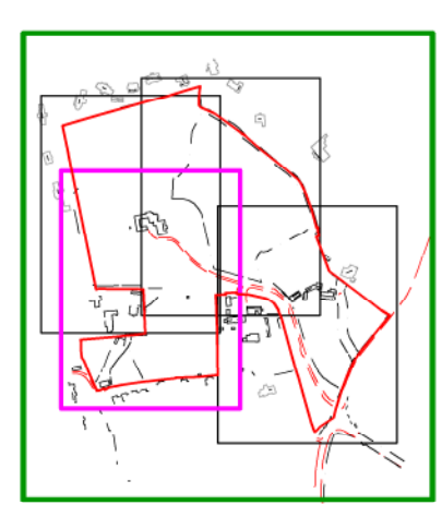
This Drawing is Copyright - © The Tree File Ltd 2021 Auburn Tree Impacts Plan South West 1/1 Scale 1:500 @ A1 This is a colour coded drawing that will be difficult or impossible to interpret if reproduced in black and white
